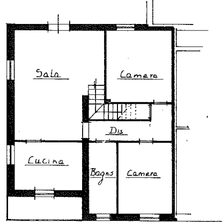
PIANO TERRA H=2.70 ml
